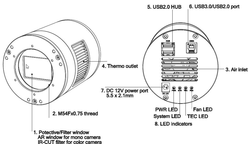
Figure 9 Camera Outline and Interface.
