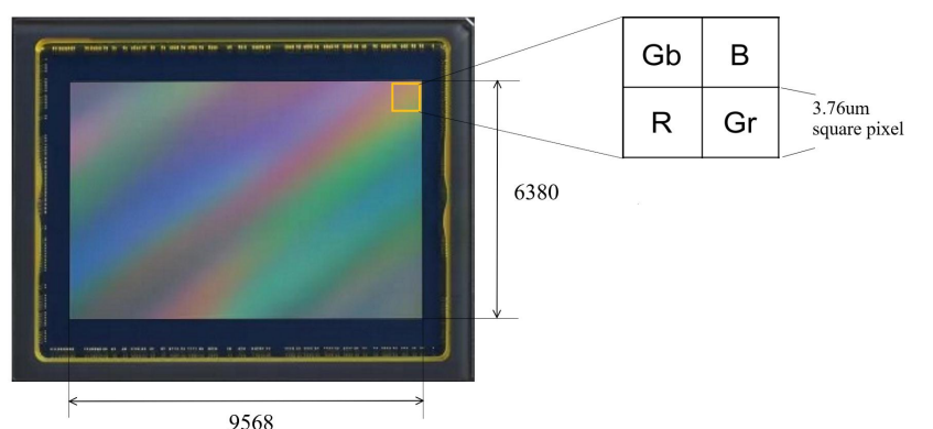
Figure 1 IMX455 Sensor and Its Pixel Structure
