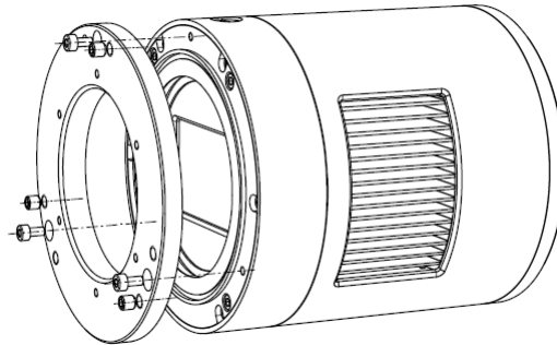
Figure 12 Tilt Adjustment
