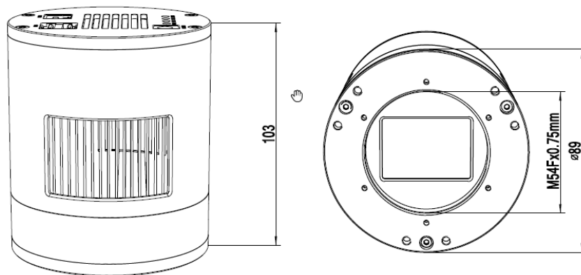
Figure 8 Dimension and Mount of SkyEye24AC
