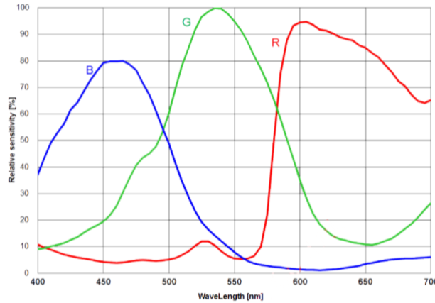
Figure 2 IMX410 Sensitivity Spectral Characteristic
