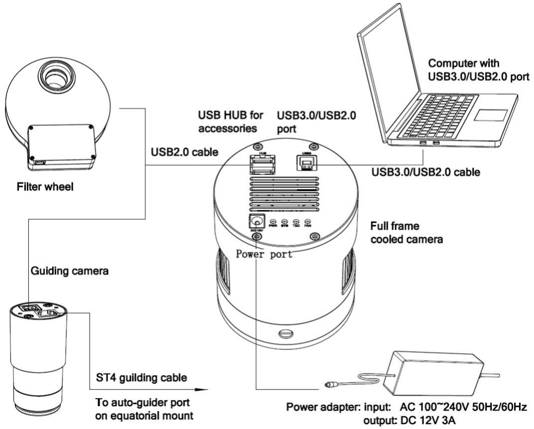
Figure 13 Camera Electric Connection
