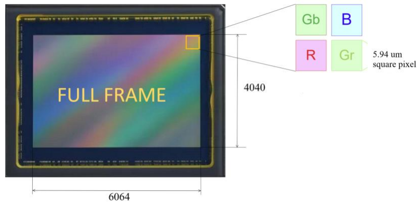
Figure 1 IMX410 Sensor
