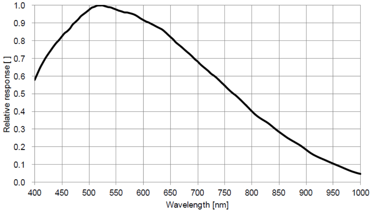
Figure 1 IMX 249 Spectral Sensitivity Characteristic
