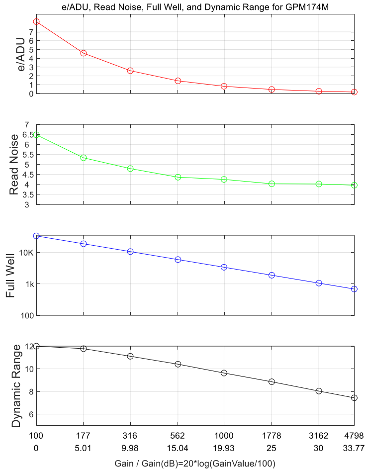
Figure 2 e-/ADU, Read Noise, Full Well and Dynamic Range for GPM174M
