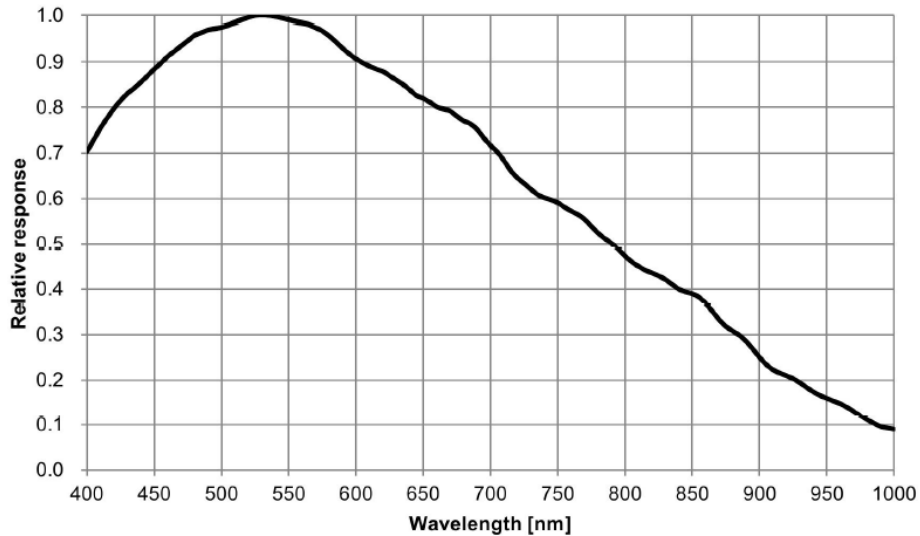
Figure 1 IMX178 Spectral Sensitivity Characteristic
