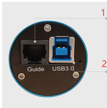
Figure 5 Camera Outline and Interface.
