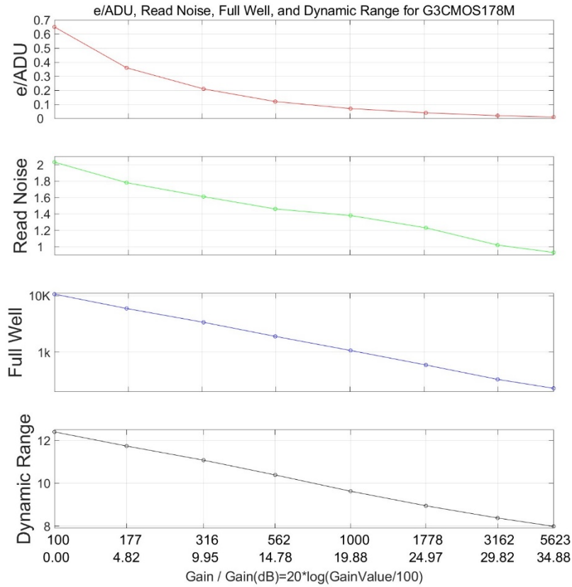
Figure 2 e-/ADU, Read Noise, Full Well and Dynamic Range for G3M178M
