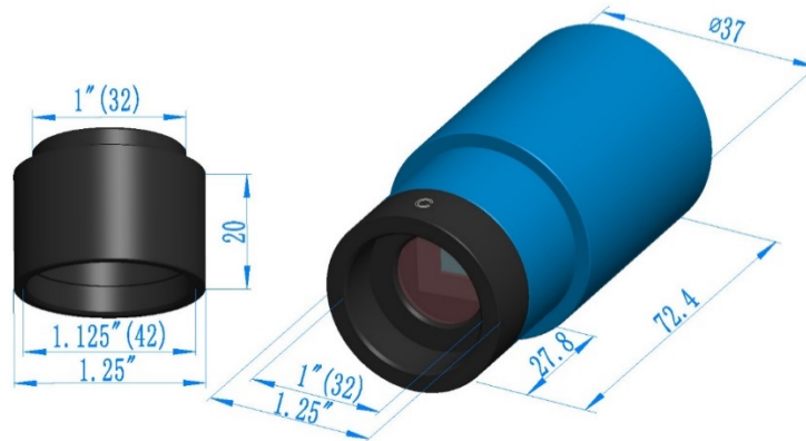
Figure 4 Dimension and Mount of G3M178C and 1.25” extender
