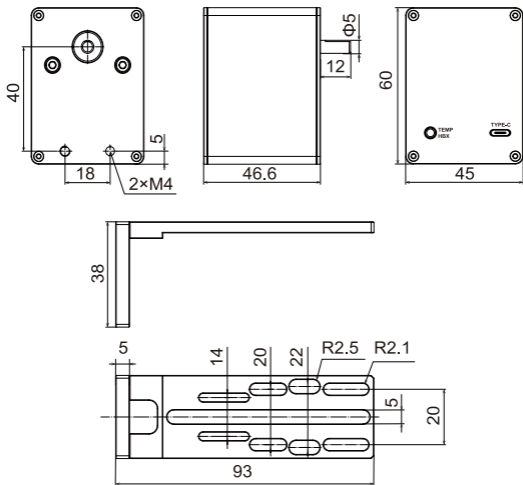
AAF ( Accessory ) Dimensions and Interface Description
